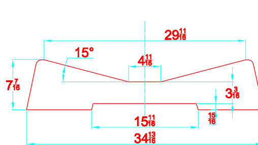
TRANSVERSAL SECTION "A" SECCION TRANSVERSAL "A"
